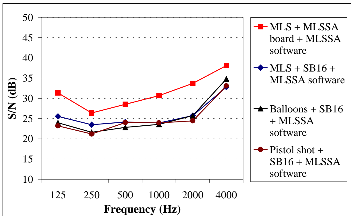
Fig. 4. Comparison between the signal-to-noise ratios obtained with different measurement techniques (hall 1).
