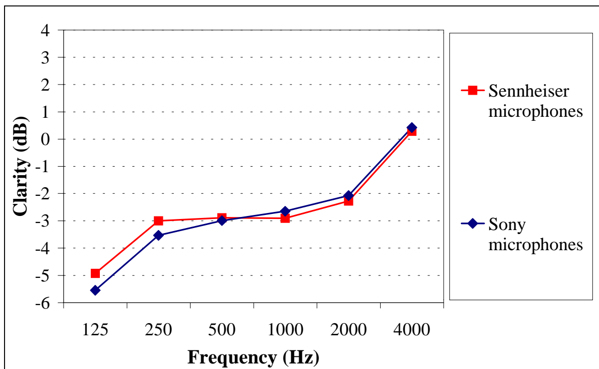
Fig. 6. Comparison between the values of the Clarity C80 obtained with two different binaural microphones (hall 2).
