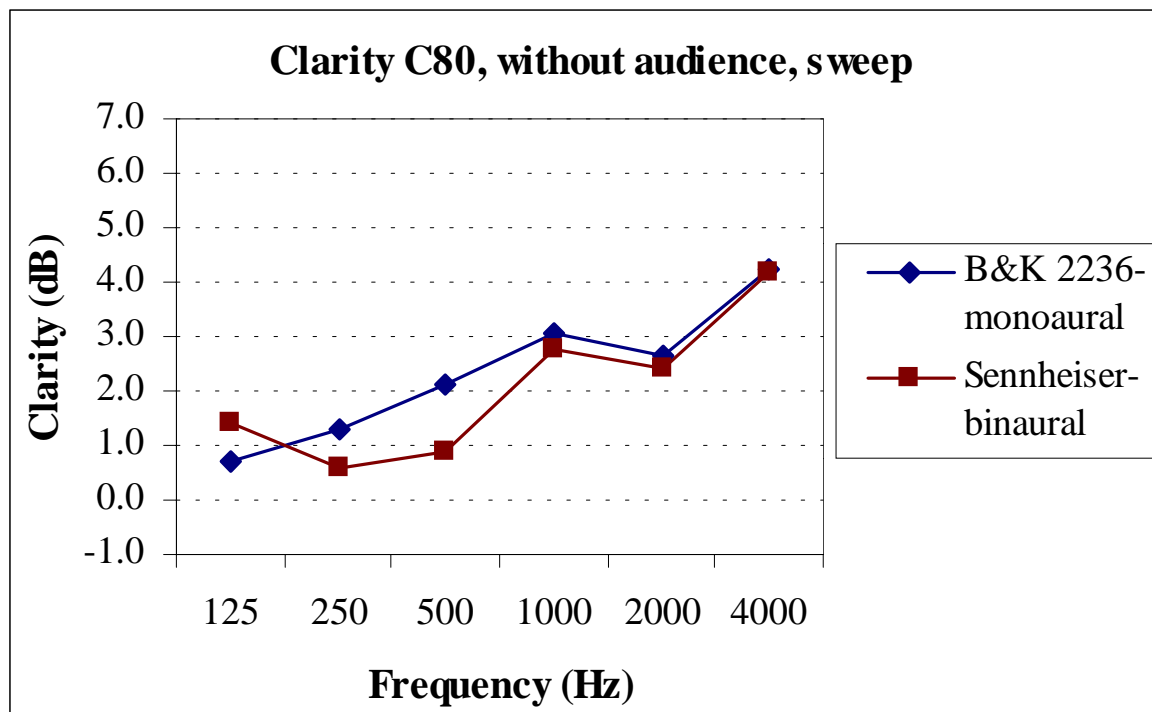
Fig. 8. Comparison between the Clarity C80 obtained from a monoaural measurement and an average of a left and right channels of a binaural measurement (hall 3).
