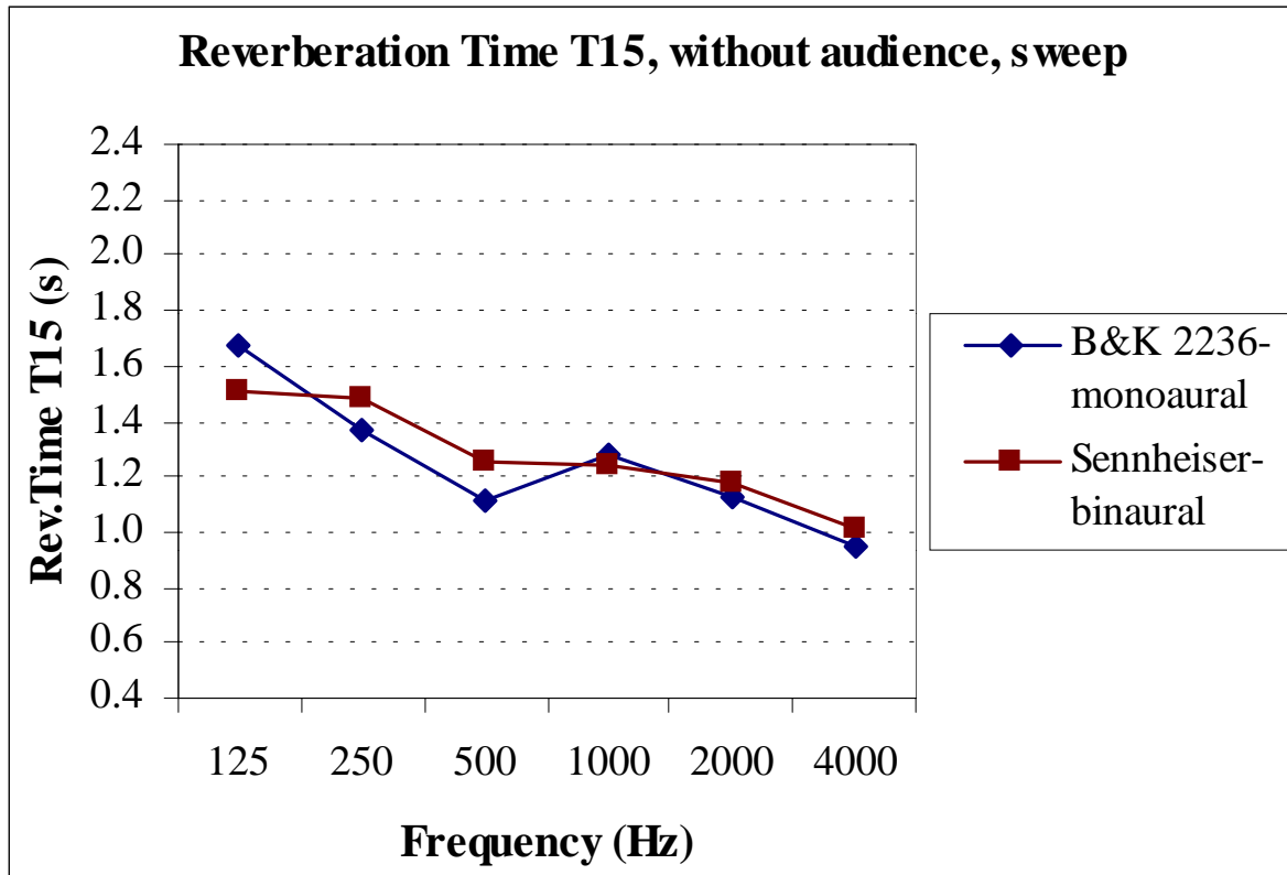
Fig. 9. Comparison between the Reverberation Time (T15) obtained from a monoaural measurement and an average of a binaural measurement (hall 3).
