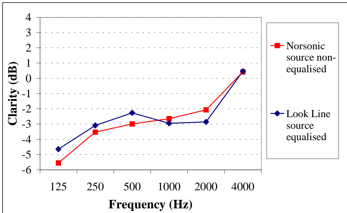
Fig. 5. Comparison between the values of the Clarity C80 obtained with two different dodechaedron sound sources one of which with an electronic equalisation (hall 2).
