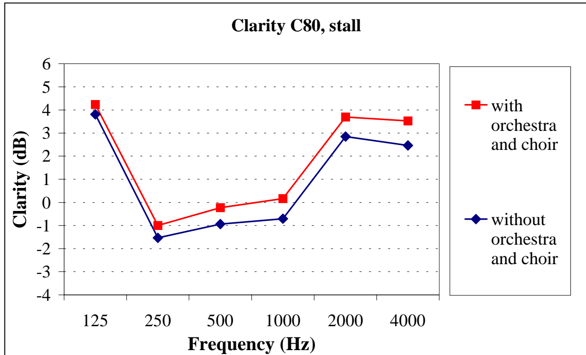
Fig. 10. Comparison between the values of the Clarity C80 obtained with and without the presence of the musicians inside the orchestra shell (hall 3).
