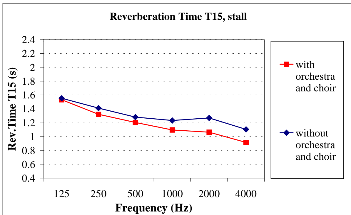
Fig. 11. Comparison between the values of the Reverberation Time obtained with and without the presence of the musicians inside the orchestra shell: the source was in the position of the first violin and the receiver was in the fourth row of the stall (hall 3).
