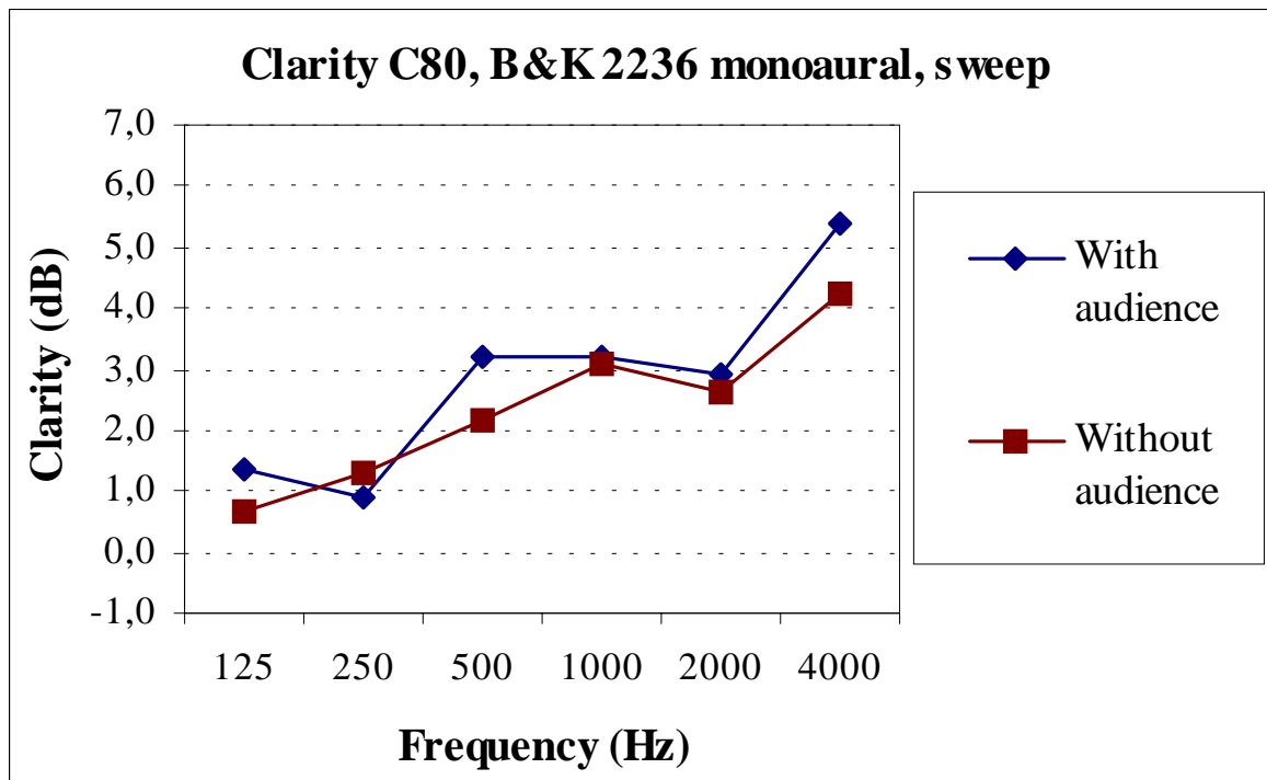
Fig. 12. Comparison between the values of the Clarity C80 with and without the audience in the hall (hall 3).
