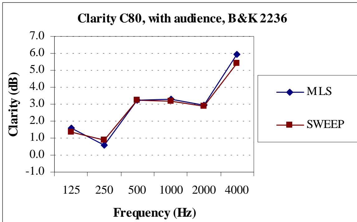
Fig. 7. Comparison between the values of the Clarity C80 obtained with the two measurement techniques (hall 3): deterministic pseudo random-signal (MLS) and exponentially-sweeping sine wave signal (SWEEP).
