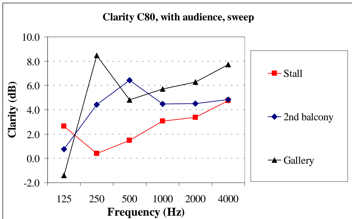
Fig. 14. Comparison between the values of the Clarity C80 obtained in three different position of the hall 3.
