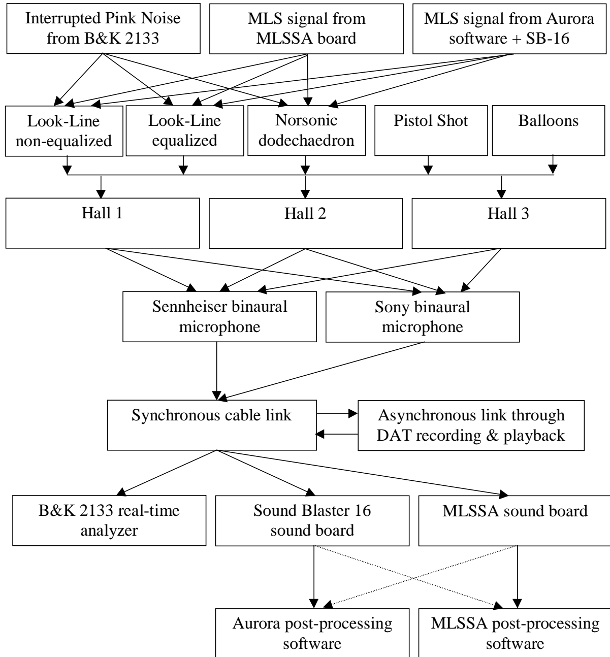
Fig. 2. Block diagram of the instruments and measurement techniques employed
