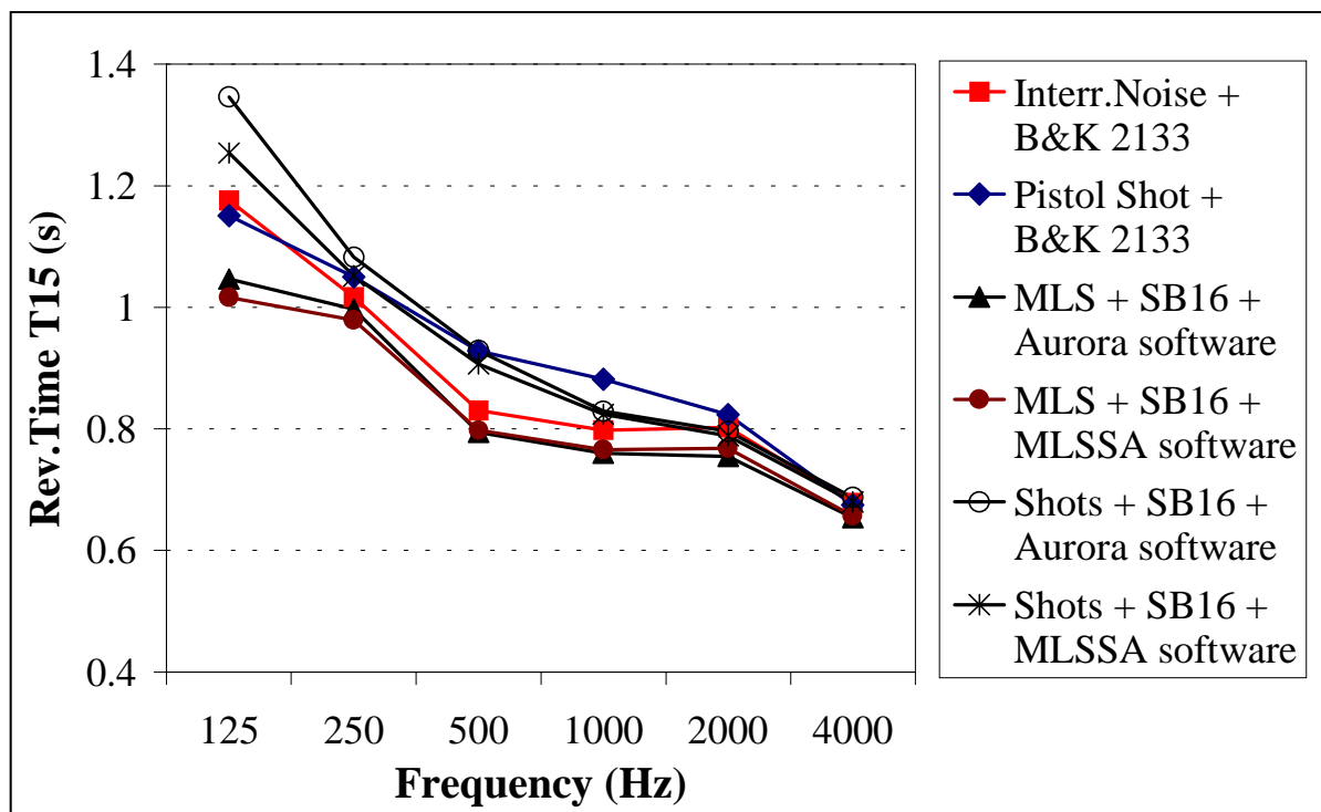
Fig. 3. Comparison between the Reverberation Times measured with the interrupted-noise method and with the backward integrated impulse responses (hall 1).
