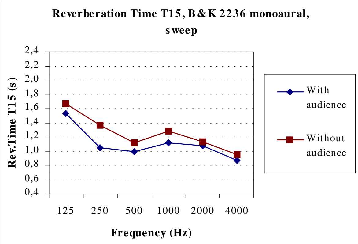
Fig. 13. Comparison between the values of the Reverberation Time T15 with and without the audience in the hall (hall 3).
