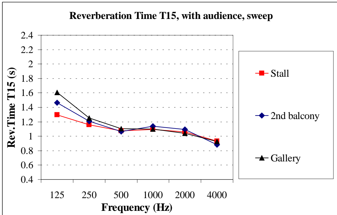
Fig. 15. Comparison between the values of the Reverberation Time T15 obtained in three different position of the hall 3.
