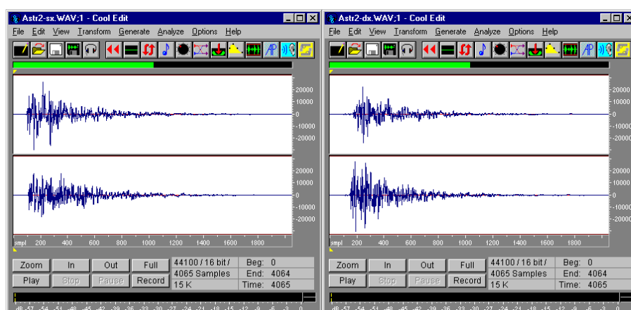
Fig. 4 – Binaural impulse responses of a car audio system (Astra)
