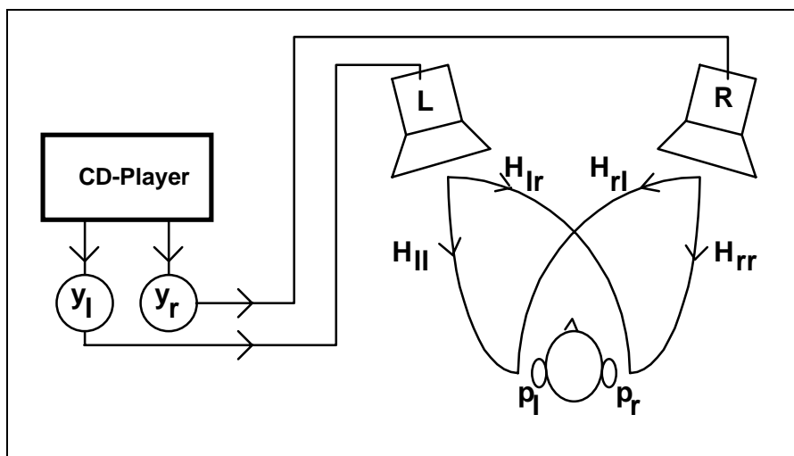
Fig. 2 – Scheme of the loudspeakers-ears transfer functions
