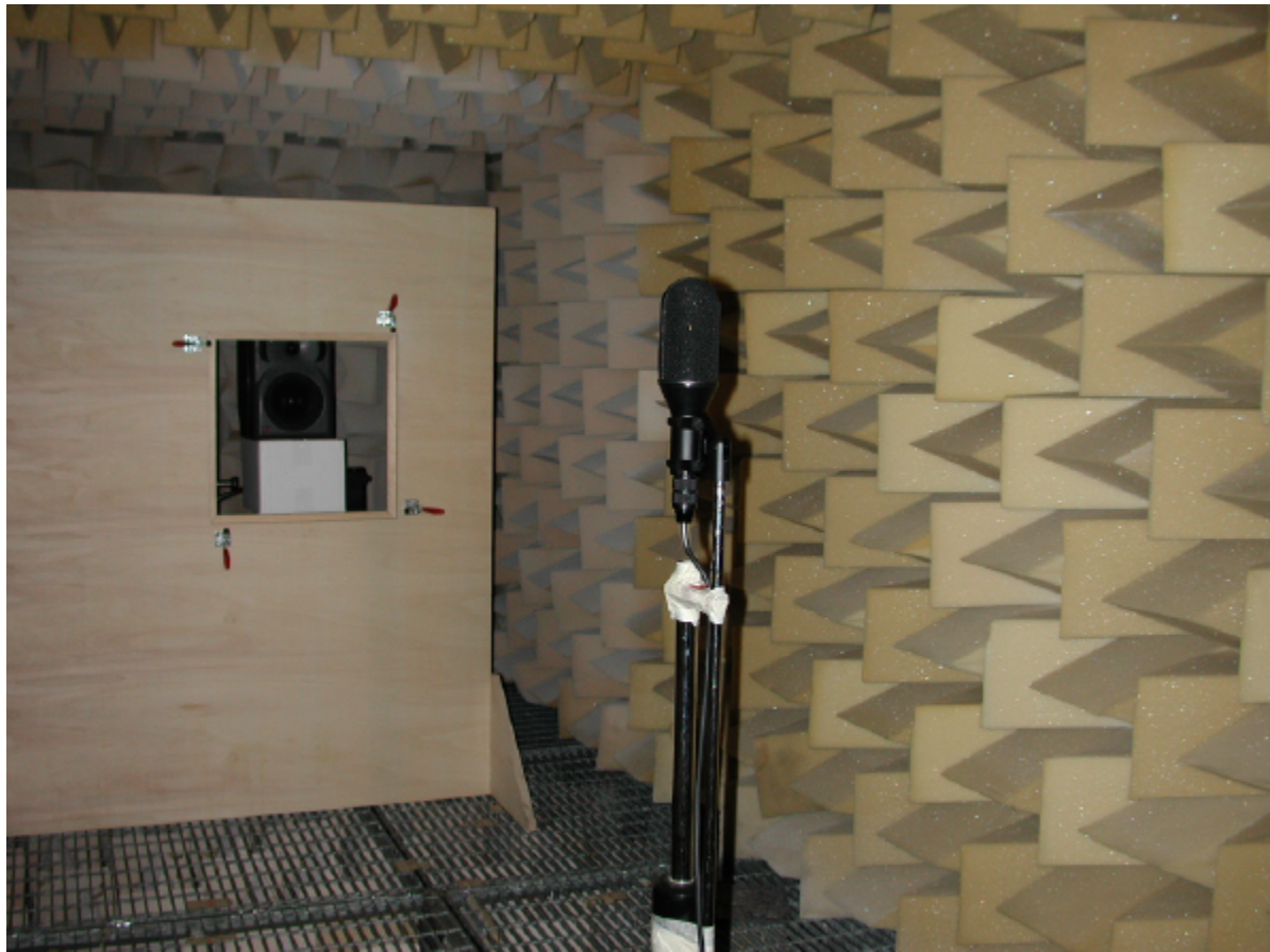
Fig. 1 – The Soundfield St-250 and the loudspeaker, in the WX and WY mounting mode.
